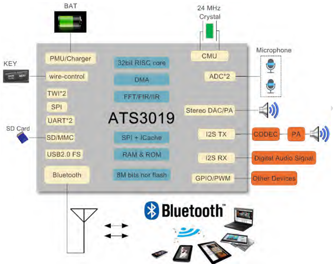
Figure 1-1 ATS3019 Application Diagram
