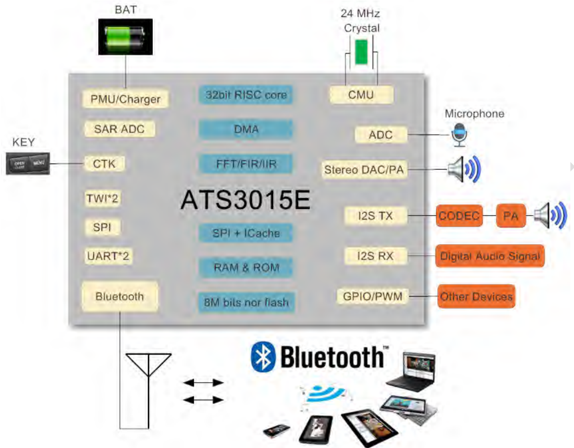
Figure 1-1 ATS3015E Application Diagram
